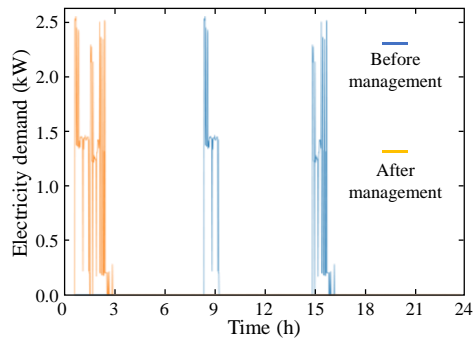
Fig. 8. Example of electricity consumption management of a washing machine using a smart plug.
